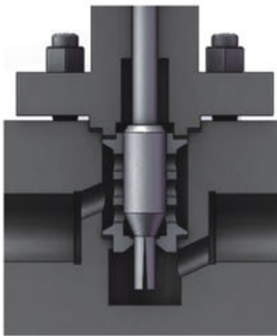
03PP Series with Trim for Low Flow Rate
