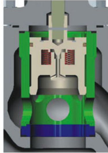
06 PM Series Pressure Relieving Trim
