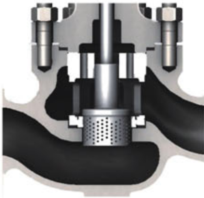
01 PP Series with Single Cage of Low Noise
