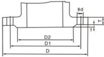
Class 150lb ( RF ) Flange
