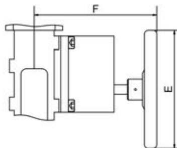
▲ Side-mounted Handwheel
