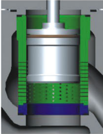
01 PM Series Single Cage of Noise Reduction
