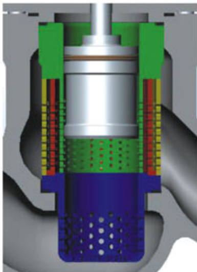
03 PM Series Multi-hole and Multistage Plating Trim of Pressure and Noise Reduction
