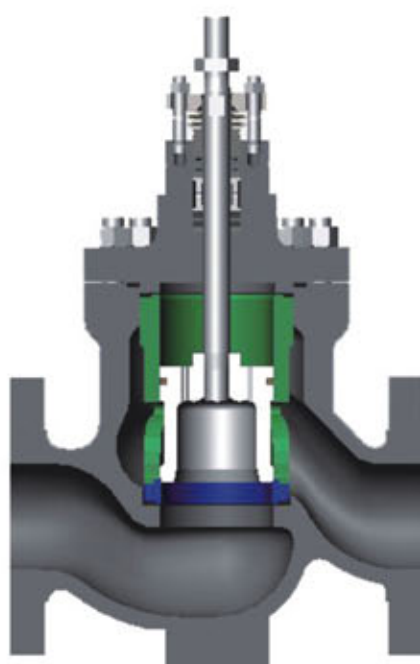
PM Series—Standard Type
