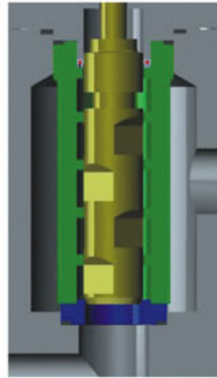
08 PM Series Multistage Plunger Trim of Pressure Reduction
