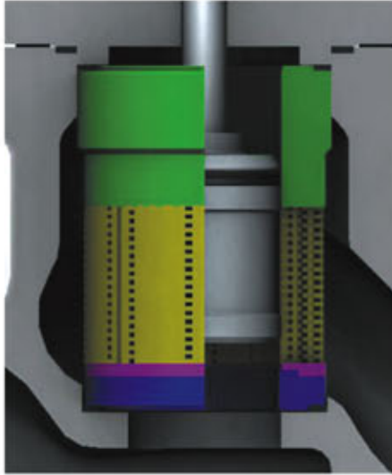
05 PM Series Labyrinth Trim
