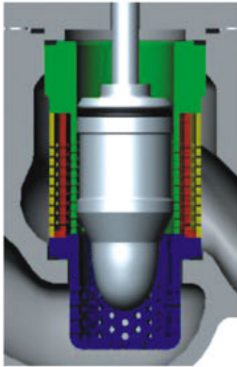
07 PM Series Multistage Trim with Plunger of Pressure Reduction
