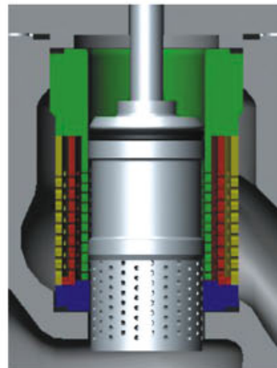
04 PM Series Multi-hole and Multistage Trim of Pressure Reduction
