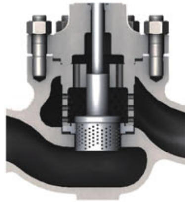
02PP Series with Double Cage of Low Noise
