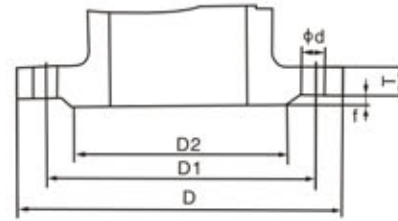
Class 300/600lb ( RF ) Flange
