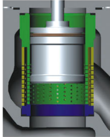
02 PM Series Double Cage of Noise Reduction
