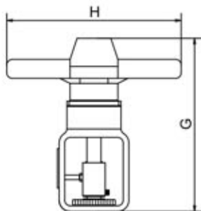
▲ Top-mounted Handwheel
