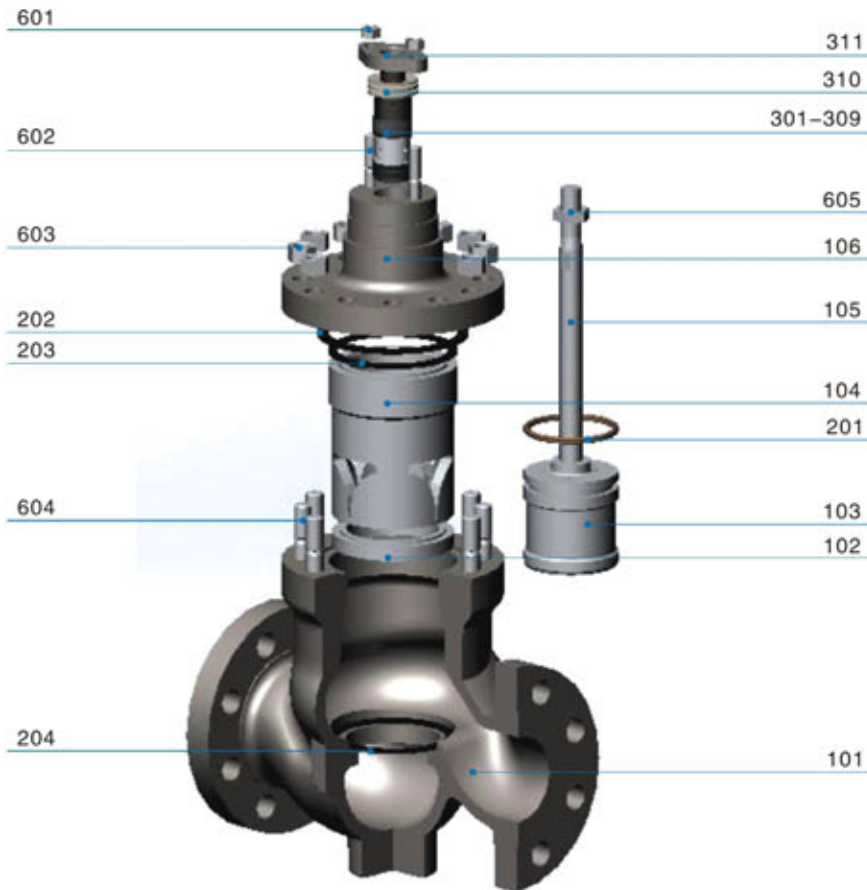
PM Series—Standard Type
