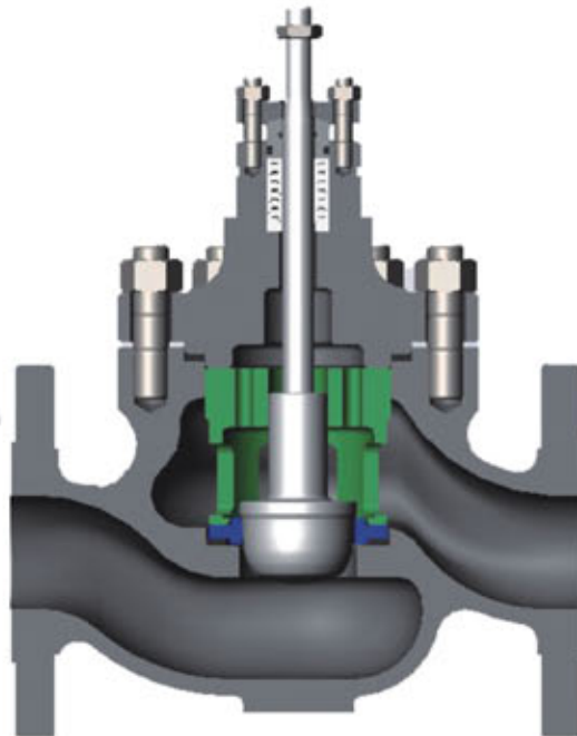
PP Series Standard Type
